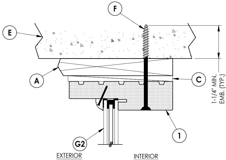
4 8 VERTICAL CROSS SECTION Shown w/ 1X Buck Outswing shown (Inswing similar)
