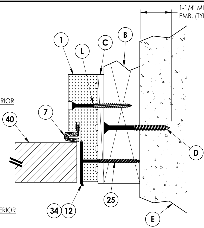
2 7 HORIZONTAL CROSS SECTION Shown w/ 2X Buck Outswing shown (Inswing similar)
